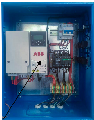
ABB variable-frequency drive
